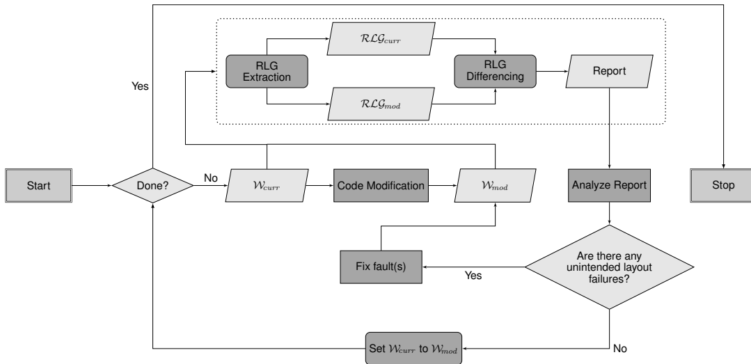
Figure 4. The main usage scenario of this paper’s approach to automatically identifying the layout regressions in a responsive web page. In this diagram, the presented approach is contained within the dotted rectangle, inputs and outputs are shown as parallelograms, the decision is depicted as a diamond and automated and manual processes are shown as rectangles with and without rounded corners, respectively (i.e., “RLG Extraction” is automated and “Analyze Report” is manual). This iterative process stops when the developer of a responsively designed web page is done fixing faults, finished making modifications to the page’s HTML and CSS, and the report suggests that there are no layout regressions. The dotted section corresponds to the internal working of REDECHECK-RM, which we expand in Figure 6.
