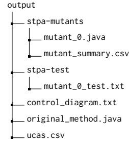
Figure 2: Output directory file structure example for m-STPA .
